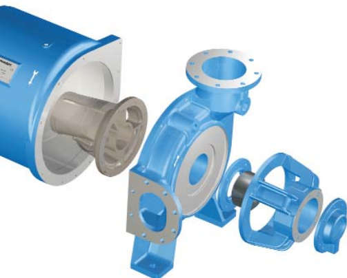
TC 8 Exploded View
